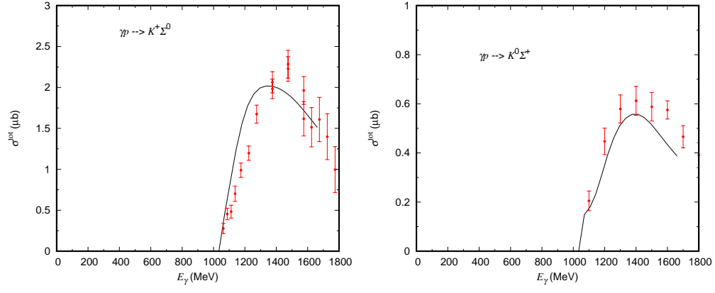
FIG. 3: \sigma^{tot} of \gamma p \rightarrow K^+ \Sigma^0, K^0 \Sigma^+
