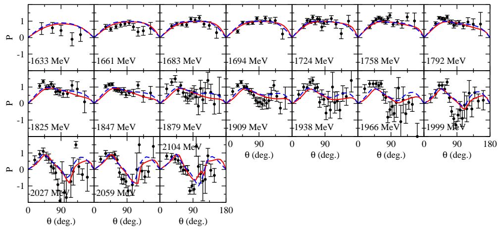
FIG. 1. Differential cross sections of \pi^- p \rightarrow K^0 \Lambda^0 .
