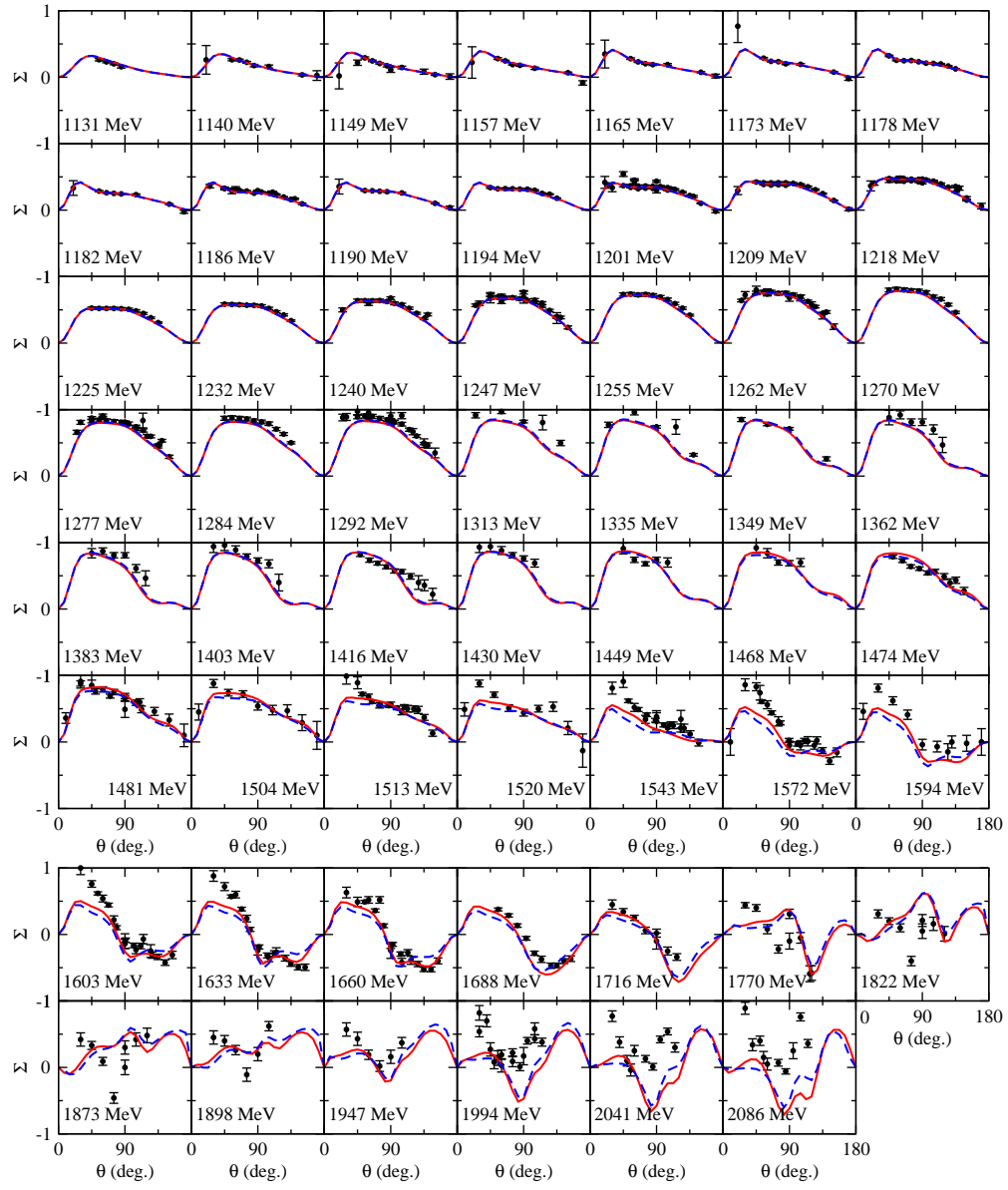
FIG. 1. The photon asymmetries \Sigma of \gamma p \rightarrow \pi^+ n . The red solid curves are the current results while the blue dashed curves are from our previous analysis.
