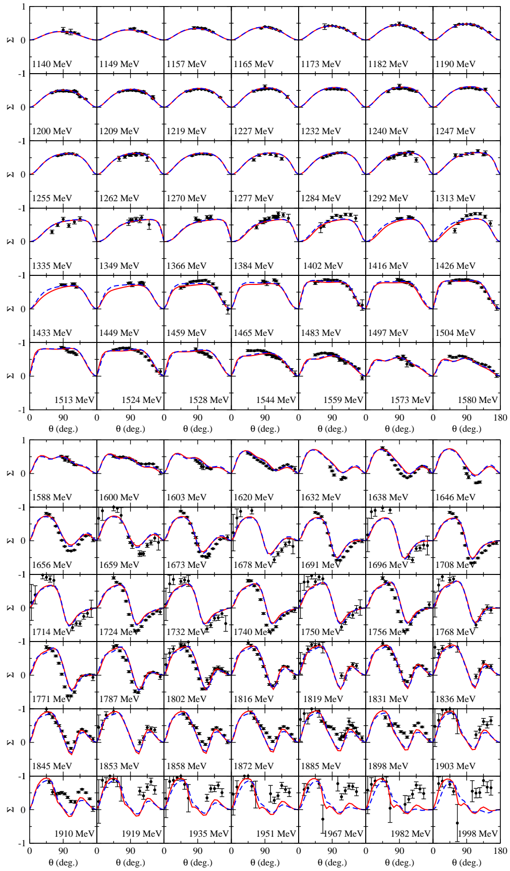
FIG. 1. The photon asymmetries \Sigma of \gamma p \rightarrow \pi^0 p .
