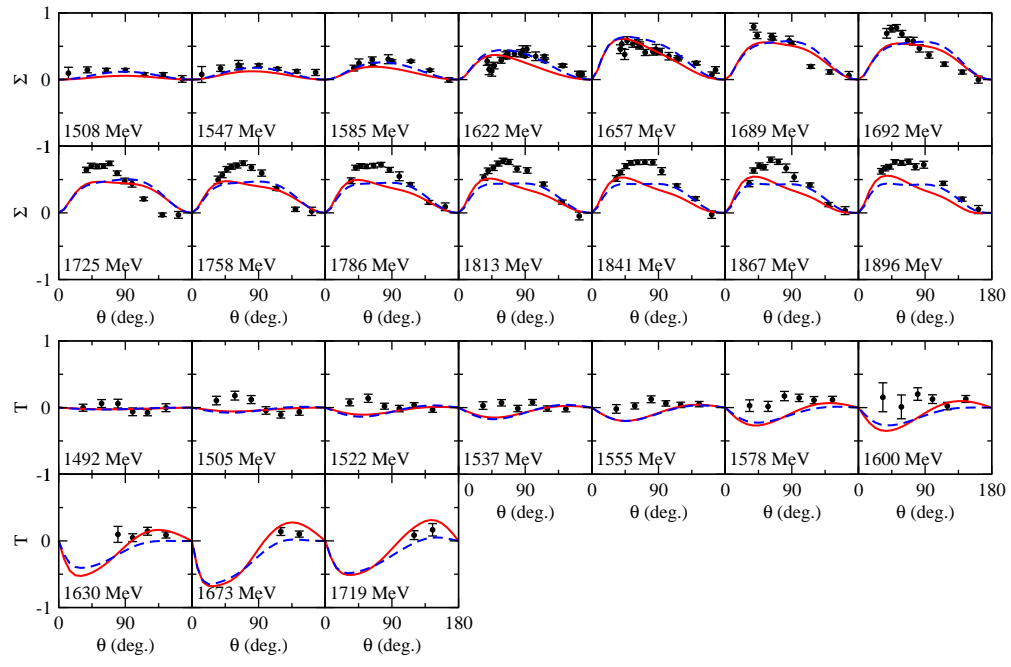
FIG. 1. \Sigma and T of \gamma p \rightarrow \eta p .
