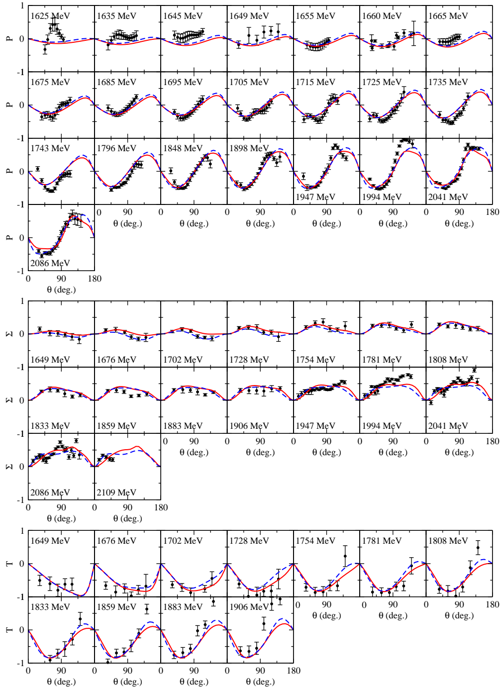
FIG. 1. Observables P , \Sigma , T of of \gamma p \rightarrow K^+ \Lambda .
