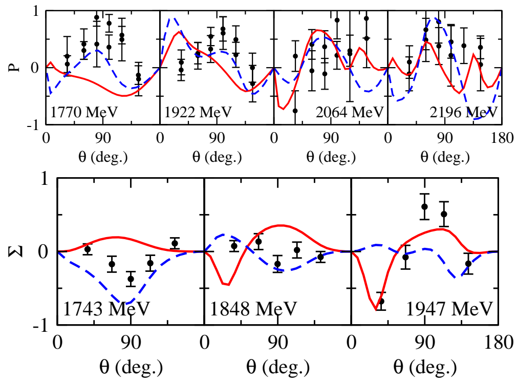
FIG. 1. P and S of \gamma p \rightarrow K^0 \Sigma^+ .
