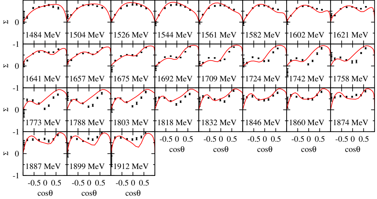
FIG. 1. Polarization \Sigma of \gamma n \rightarrow \pi^0 n .
