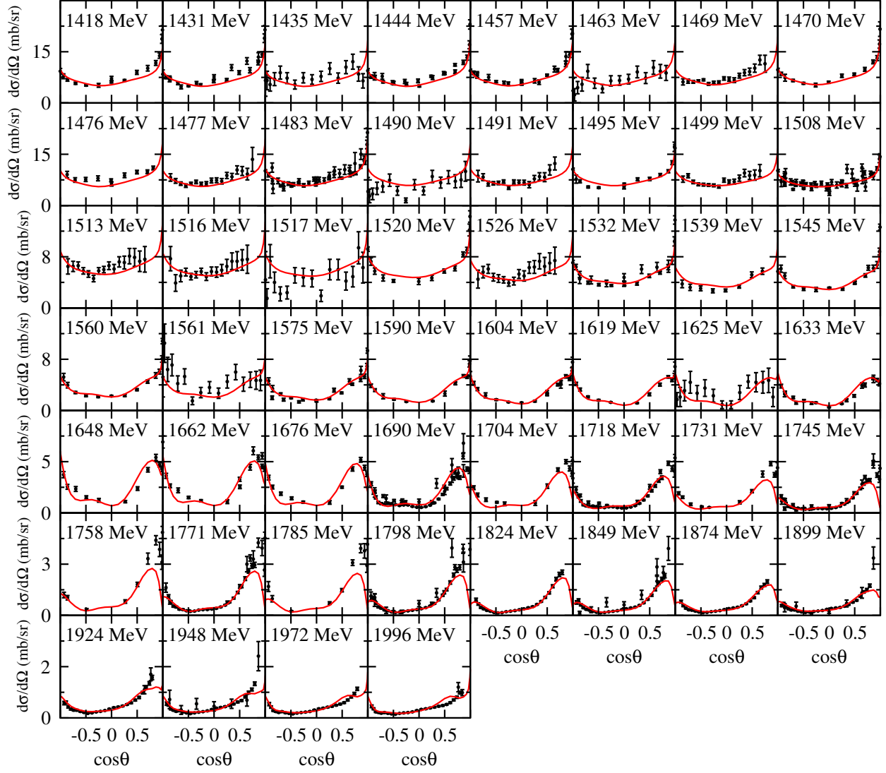
FIG. 1. Differential cross section for \gamma n \rightarrow \pi^- p .
