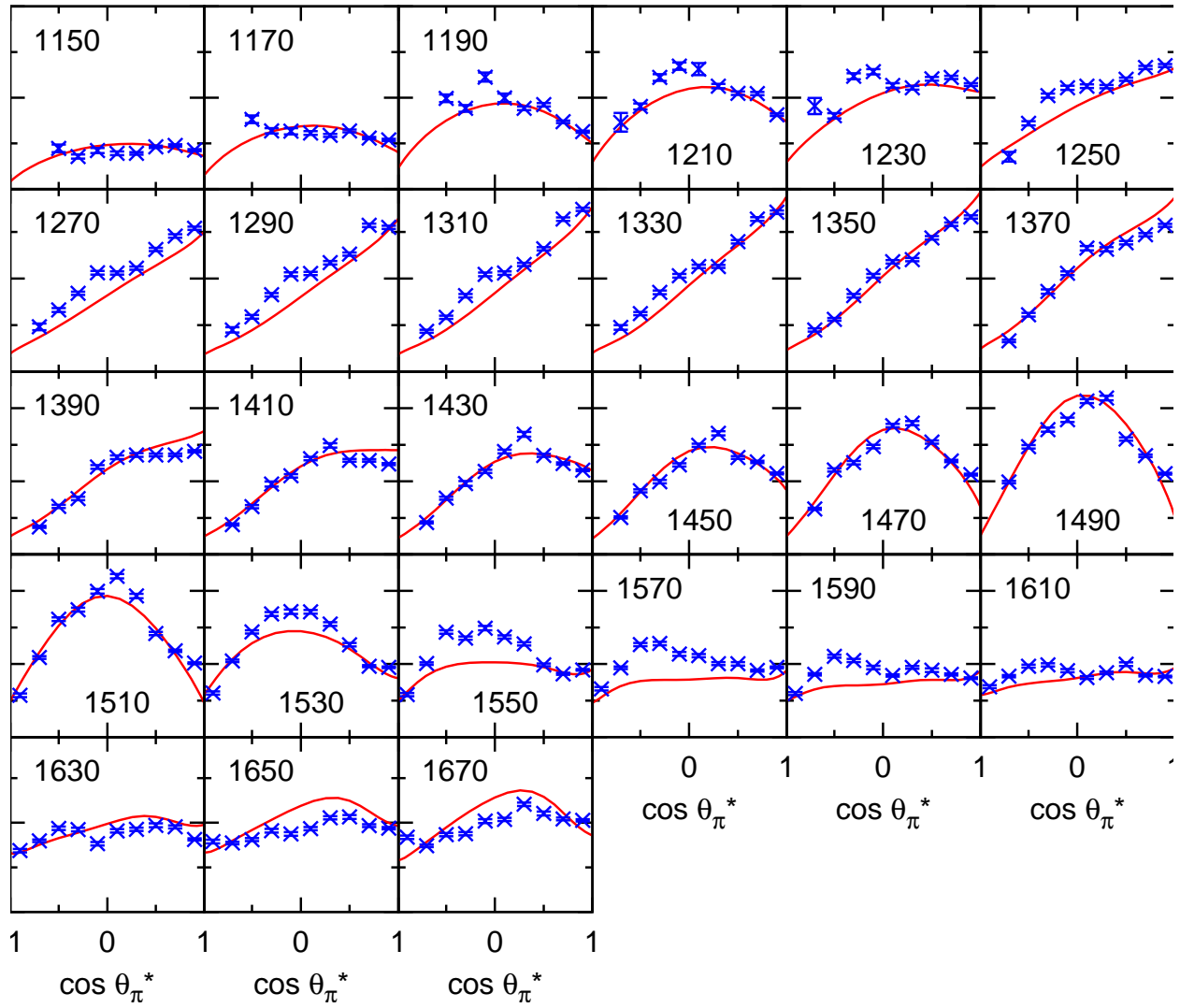
FIG. 1. Differential cross section for \gamma^*p \rightarrow \pi^+n at Q^2 = 2.91(\text{GeV}/c)^2 .
