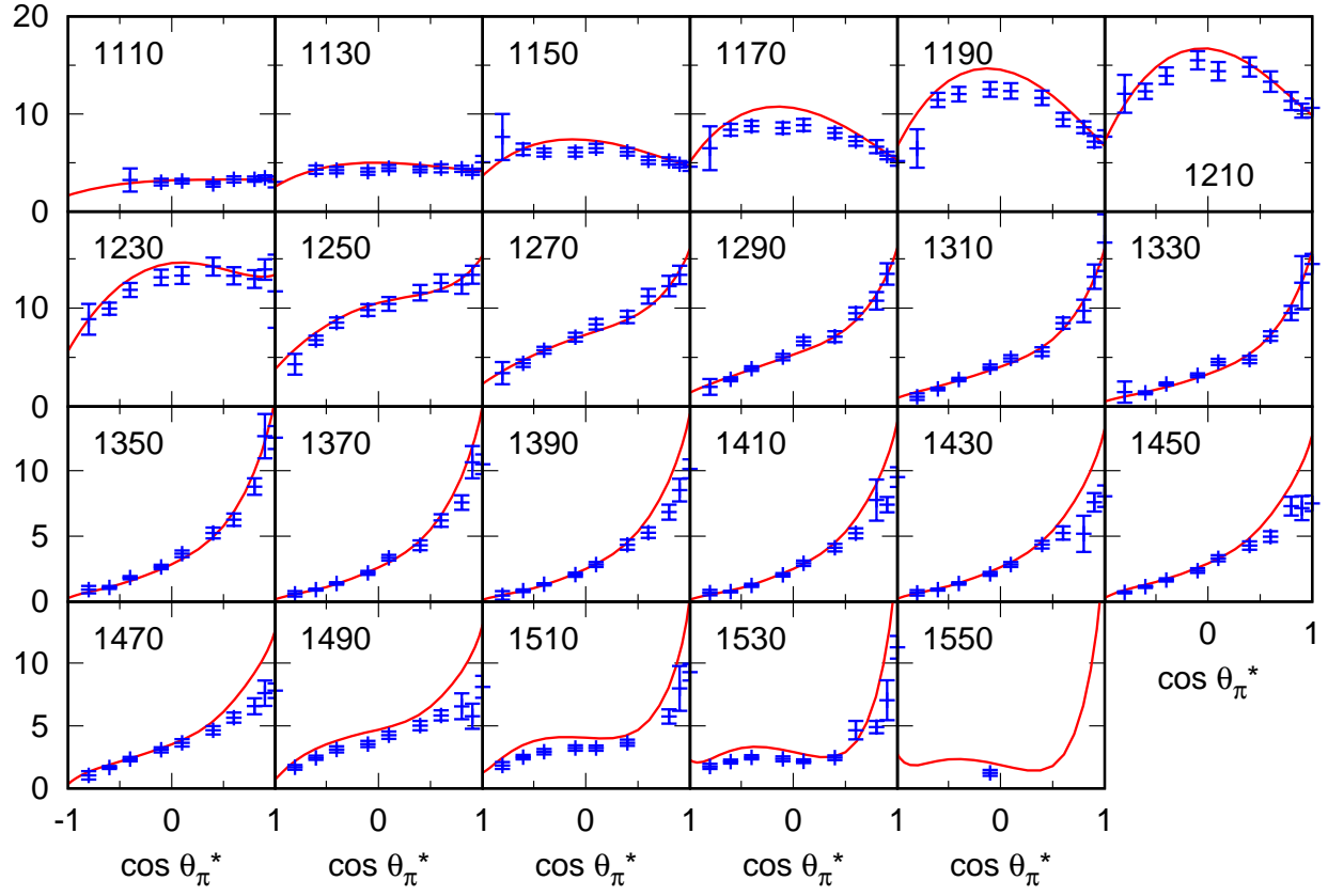
FIG. 1. Differential cross section for \gamma^* p \rightarrow \pi^+ n at Q^2 = 0.4(\text{GeV}/c)^2 .
