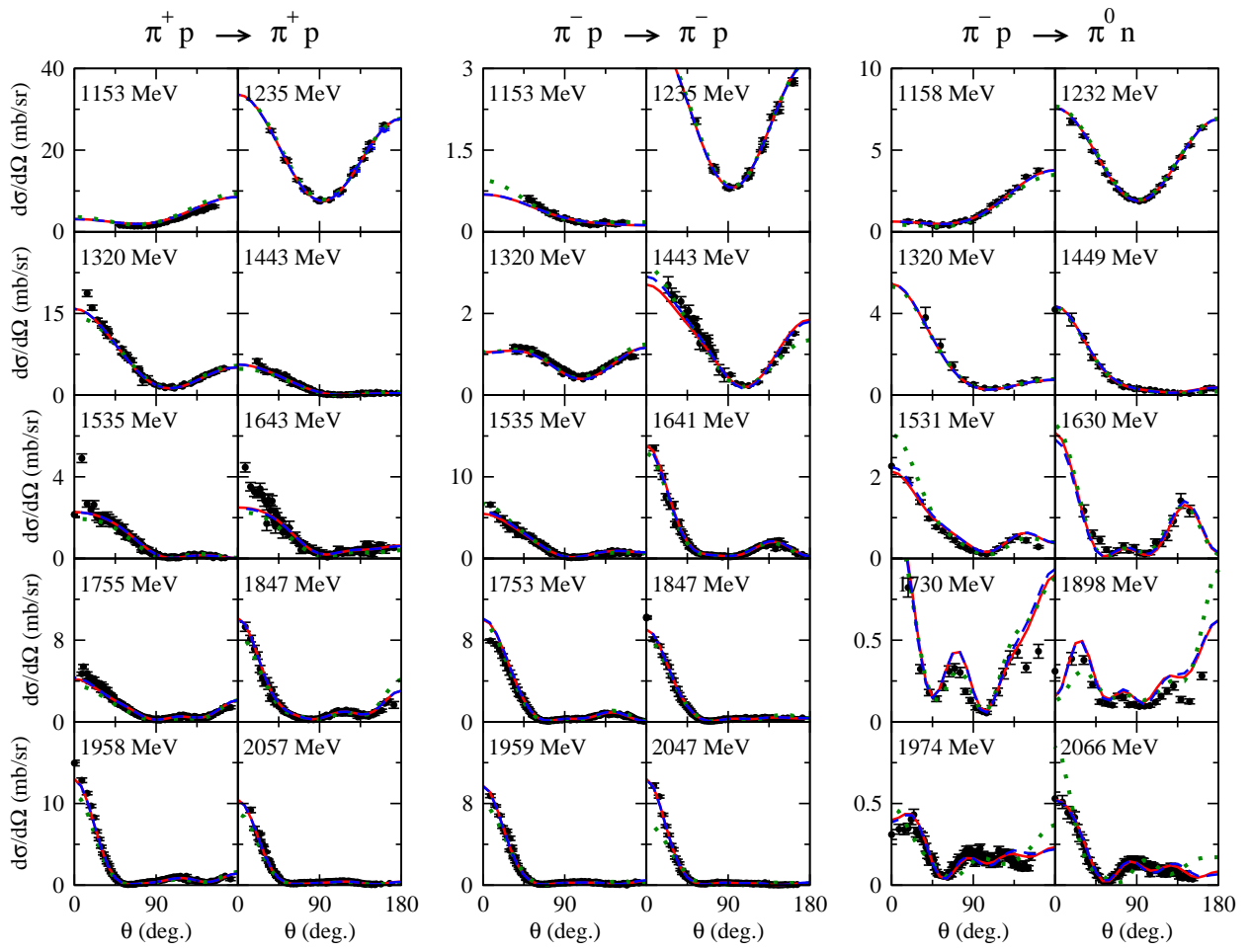
FIG. 1. Differential cross section for \pi N \rightarrow \pi N . The red solid curves are the current results while the blue dashed curves are from our previous analysis of 2007.
