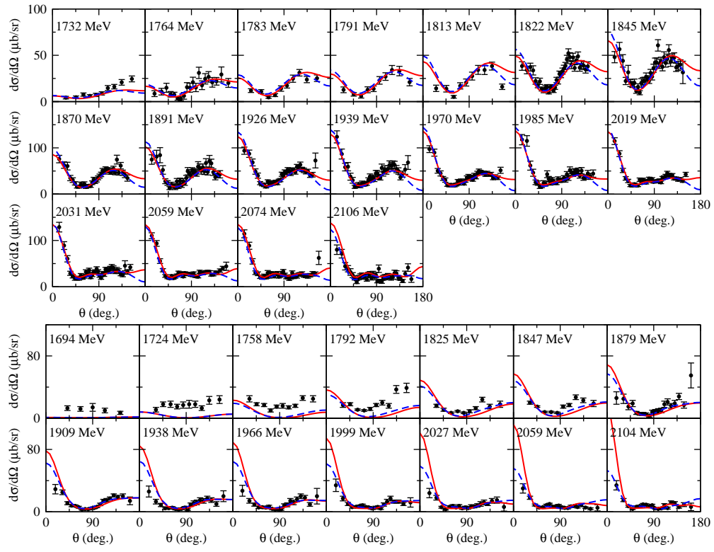
FIG. 1. Differential cross sections of \pi^+p \rightarrow K^+\Sigma^+ (upper) and \pi^-p \rightarrow K^0\Sigma^0 (lower).
