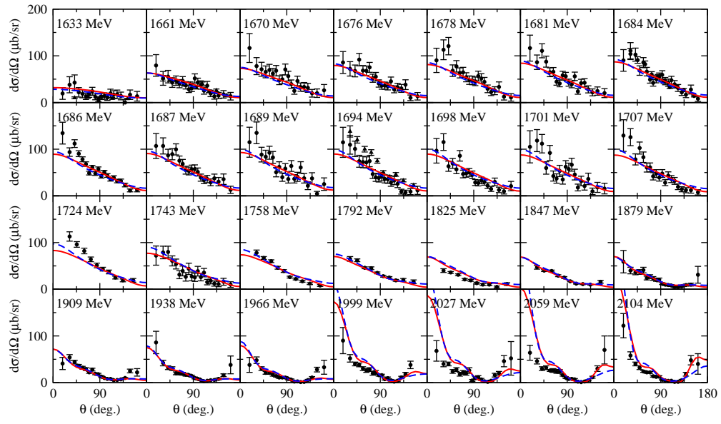
FIG. 1. Differential cross sections of \pi^- p \rightarrow K^0 \Lambda^0 .
