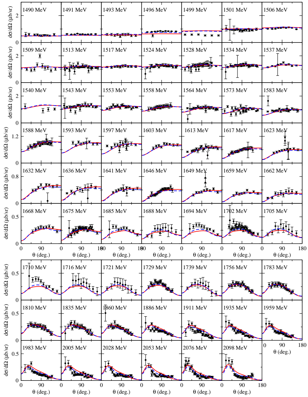
FIG. 1. Differential cross sections of \gamma p \rightarrow \eta p .
