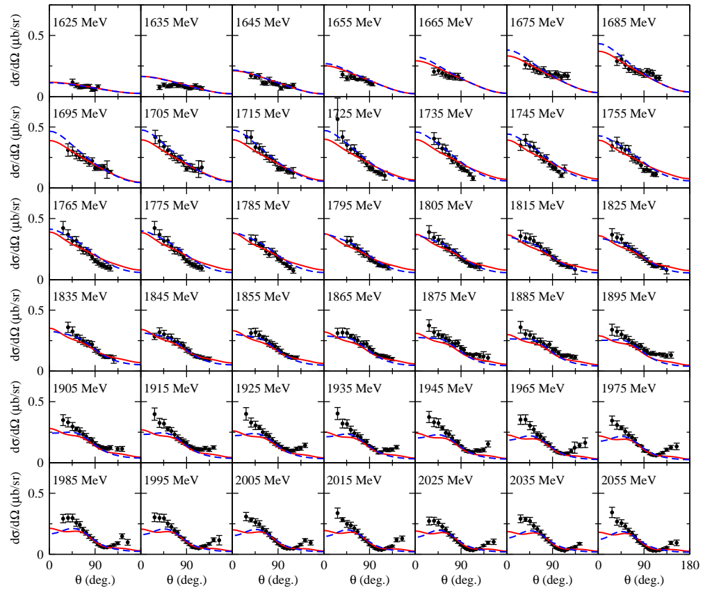
FIG. 1. Differential cross sections of \gamma p \rightarrow K^+ \Lambda .
