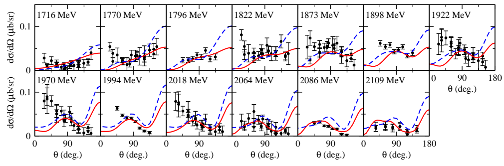
FIG. 1. Differential cross sections of \gamma p \rightarrow K^0 \Sigma^+ (lower).
