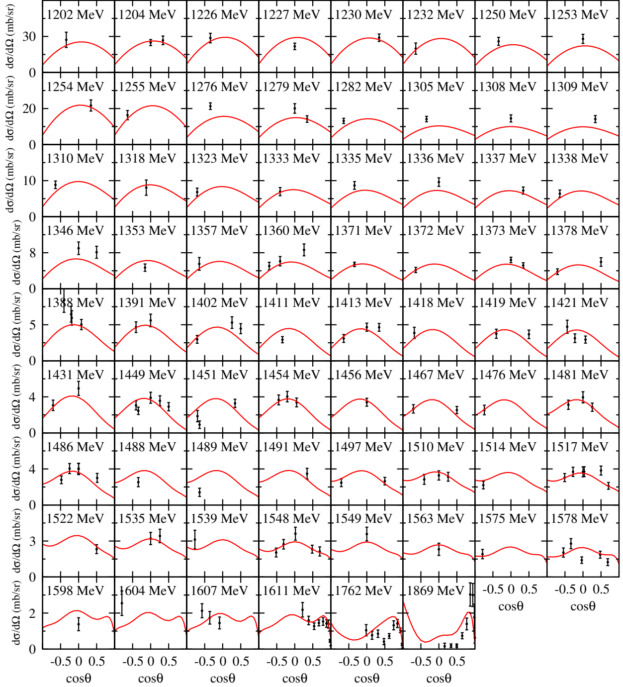
FIG. 1. Differential cross section for \gamma n \rightarrow \pi^0 n .
