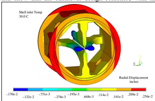
Figure 6: Radial displacements
