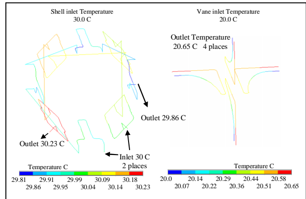
Figure 4: Coolant temperature distribution
