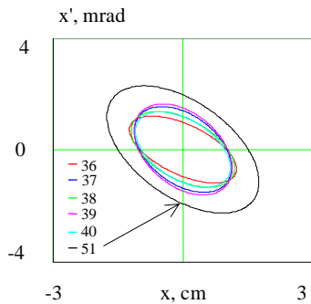
Figure 6: Vertical phase space ellipses of single charge-state beams. The black ellipse corresponds to double-stripped \text{U}^{51+} .
