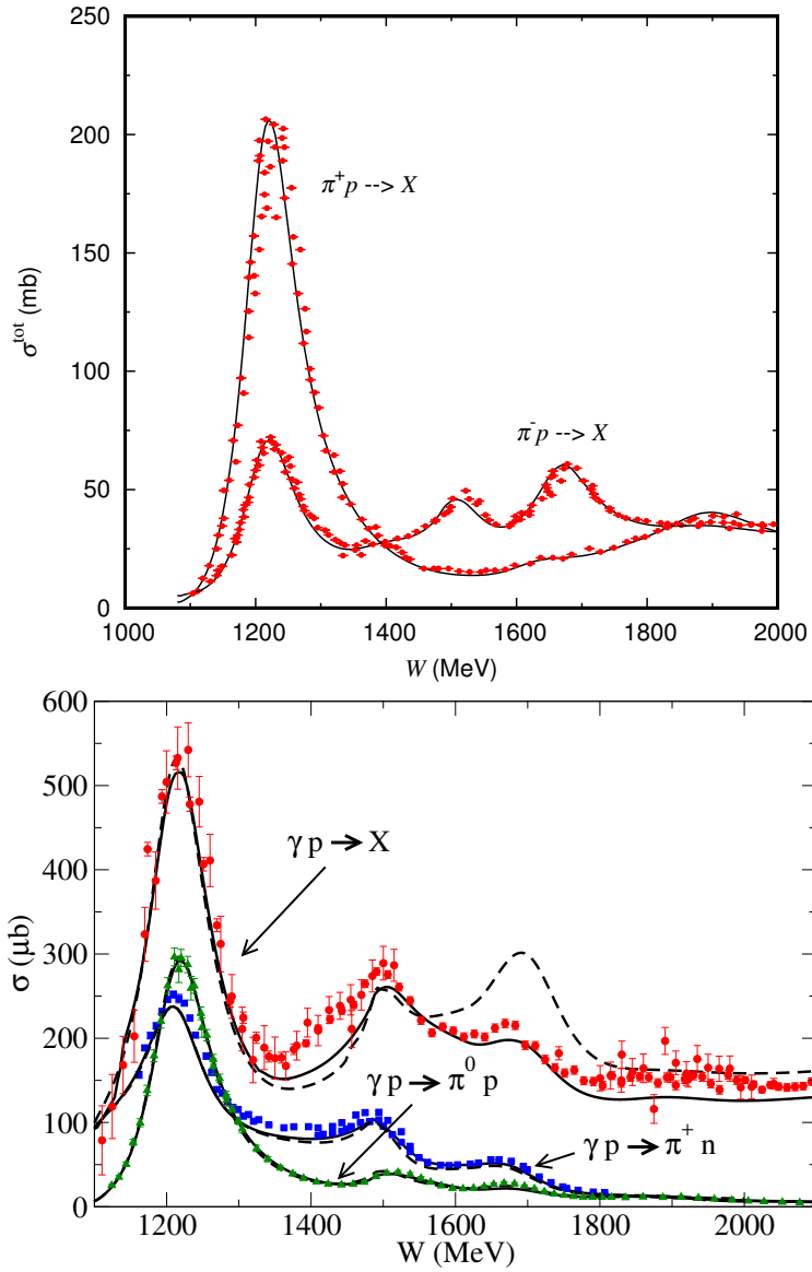
FIG. 1: \sigma^{tot} of \pi^\pm p \rightarrow X (upper) and \gamma p \rightarrow X (lower)
