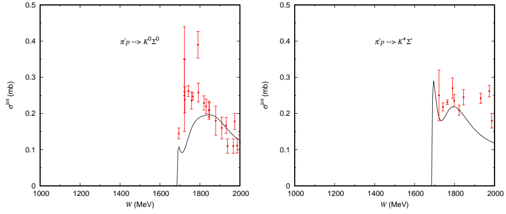
FIG. 3: \sigma^{tot} of \pi^- p \rightarrow K^0 \Sigma^0, K^+ \Sigma^-
