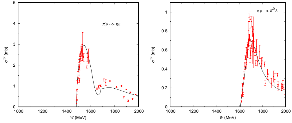
FIG. 2: \sigma^{tot} of \pi^- p \rightarrow \eta n, K^0 \Lambda
