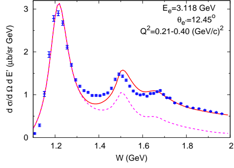
FIG. 1: Differential cross sections of p(e, e')X at Q^2 \sim 0.3(\text{GeV}/c)^2 . Dashed curves are from the contributions of p(e, e'\pi)N .
