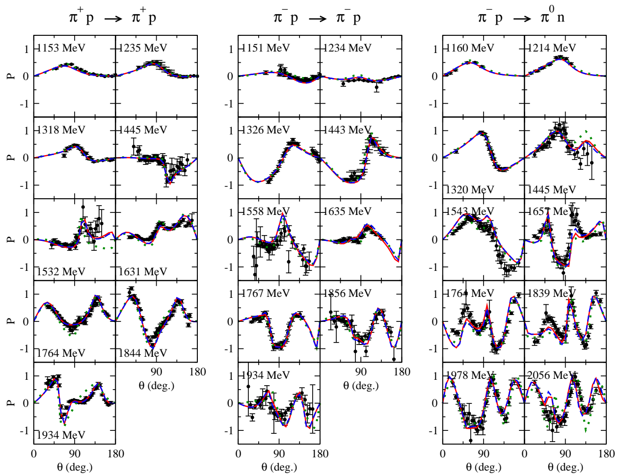
FIG. 1. The target polarization P of \pi N \rightarrow \pi N . The red solid curves are the current results while the blue dashed curves are from our previous analysis of 2007.
