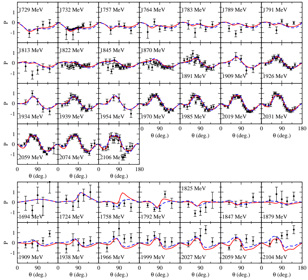
FIG. 1. Polarization P of \pi^+p \rightarrow K^+\Sigma^+ (upper) and \pi^-p \rightarrow K^0\Sigma^0 (lower).
