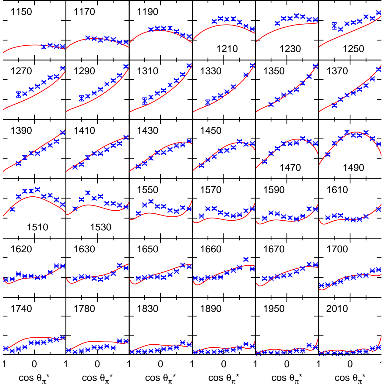
FIG. 1. Differential cross section for \gamma^*p \rightarrow \pi^+n at Q^2 = 1.76(\text{GeV}/c)^2 .
