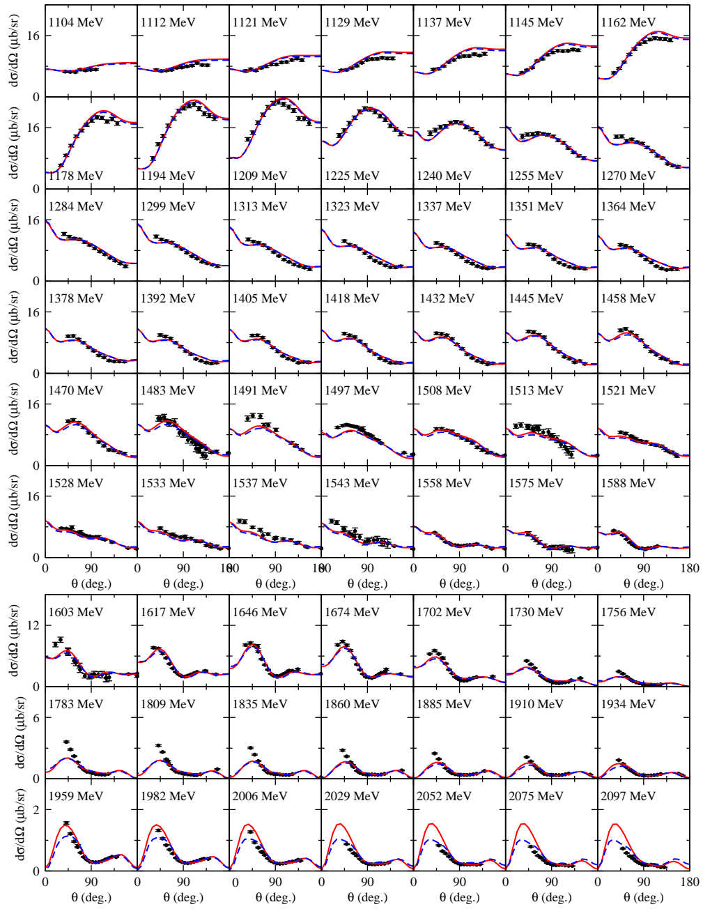
FIG. 1. Differential cross sections of \gamma p \rightarrow \pi^+ n . The red solid curves are the current results while the blue dashed curves are from our previous analysis.
