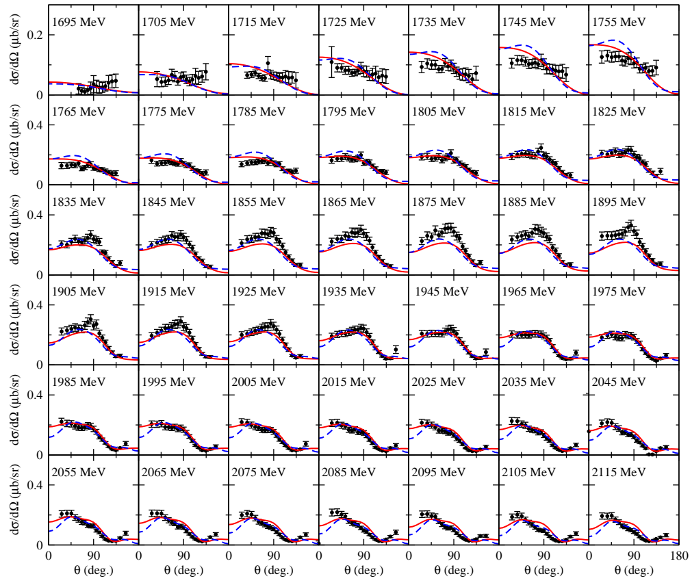
FIG. 1. Differential cross sections of \gamma p \rightarrow K^+ \Sigma^0 .
